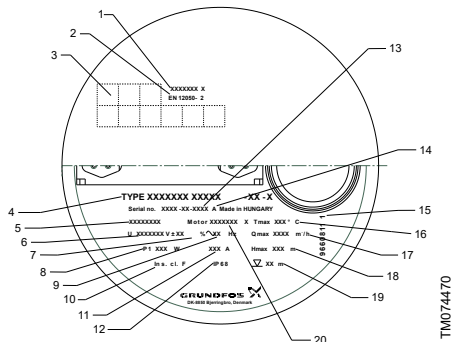
Nameplate example
