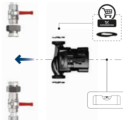
Fig. 2 Pump installation
